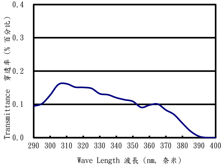
UV Transmittance Characteristics
